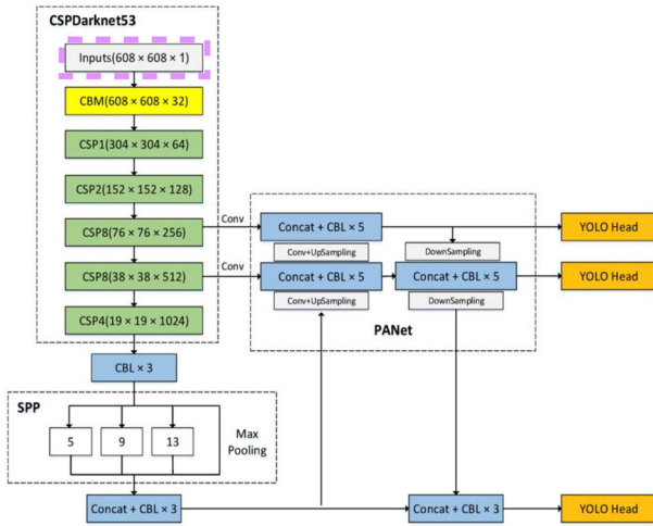
FIGURE 6. YOLOv4 architecture with the input layer (highlighted with dotted purple box) modified to accept one channel input.
