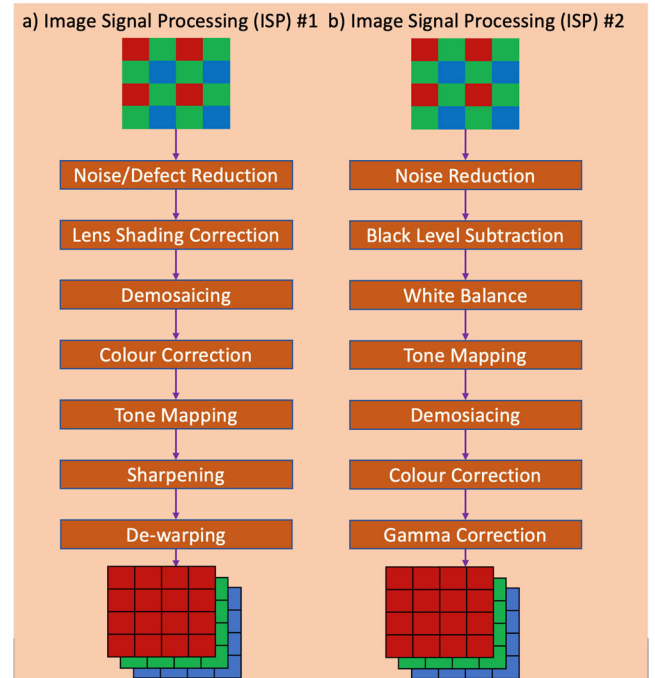
FIGURE 2. a) Some fundamental processing steps in a generic colour pipeline in an imaging sensor, and b) the ISP blocks considered in [37]. In both cases, the output is a 3 colour channel frame with the same resolution of the input Bayer data.
